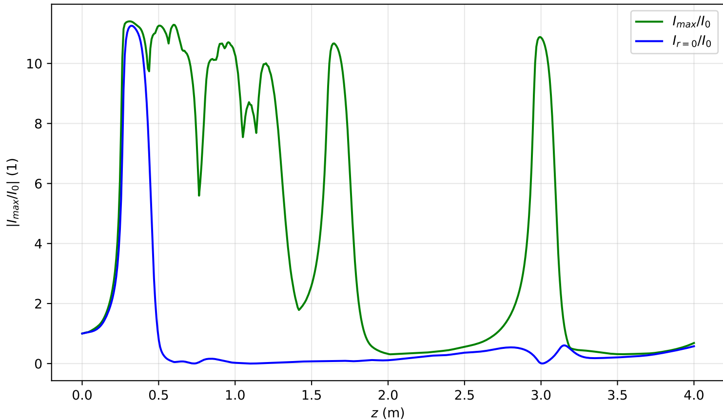
I_{max}(x = 0, y = 0, z)/I_0 , P_{in}=9.7P_{cr} , noisy input, artificial time
